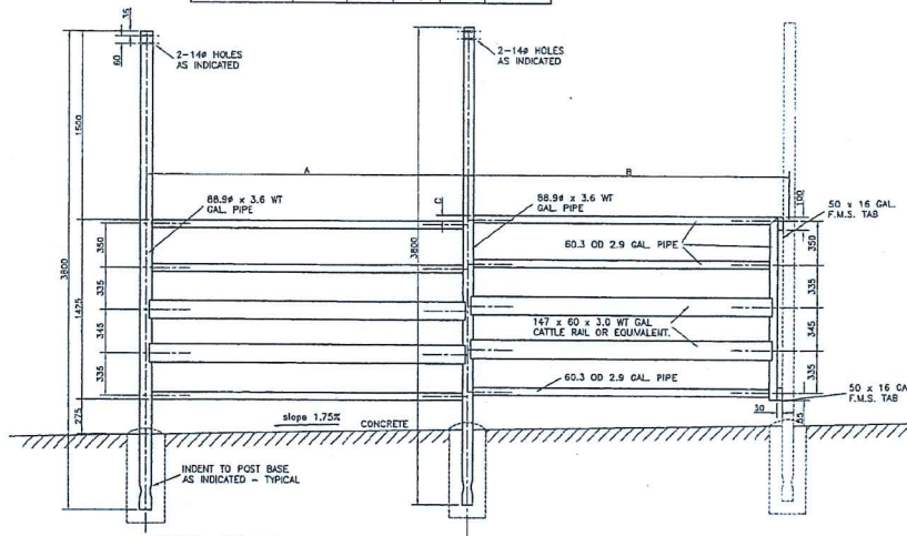
PANEL CP11A
