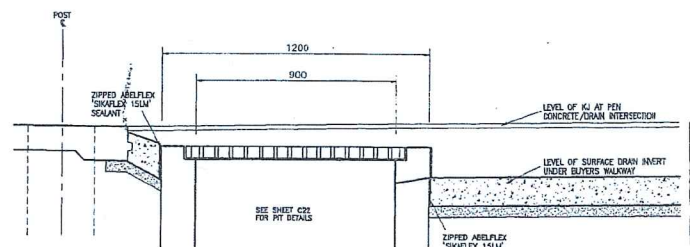
SURFACE DRAIN SECTIONAL VIEW
