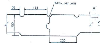
KEY JOINT DETAIL 'KJ'
