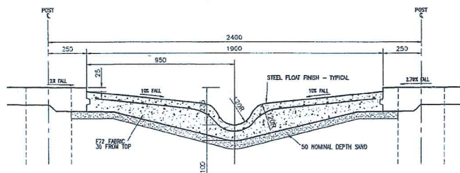
SURFACE DRAIN DETAIL UNDER BUYERS WALKWAY
