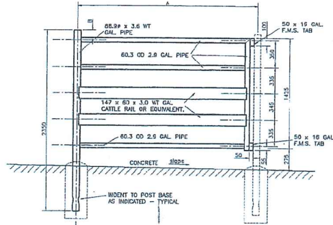
PANEL CP4A - CP4R
