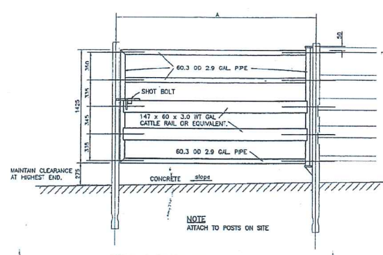
GATE CG2A
