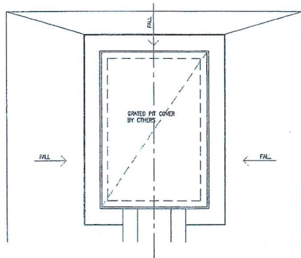
SURFACE DRAIN / PIT PLAN DETAIL
