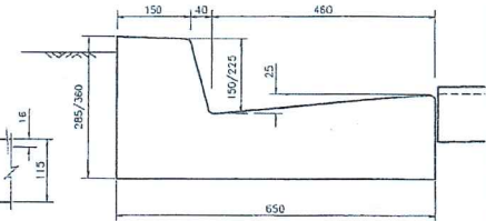
150/225 KERB & GUTTER DETAIL
