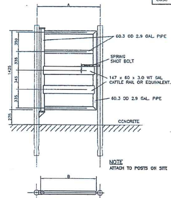
GATE CG6A
