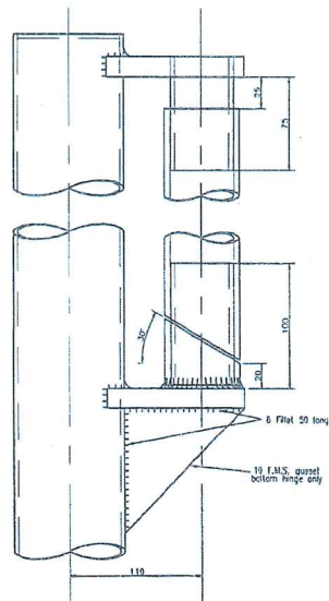
GATE CG5 HINGE DETAIL SCALE 1:2
