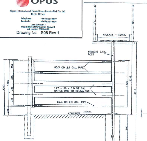
PANEL CP2A - CP2B REVERSED
