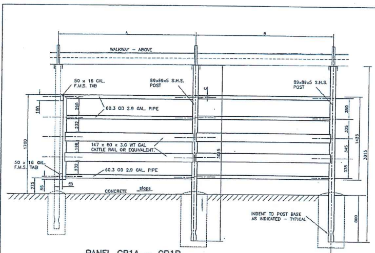
PANEL CP1A - CP1B
