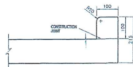
KNOCKOFF PLINTH DETAIL
