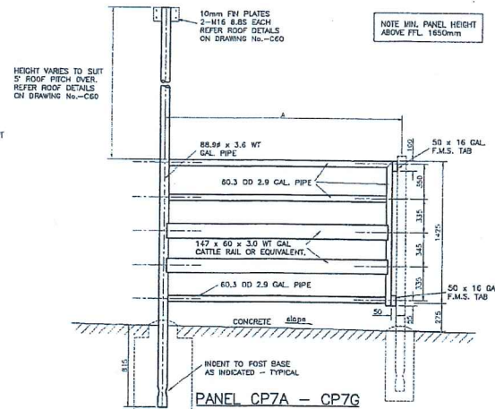
PANEL CP7A - CP7G
