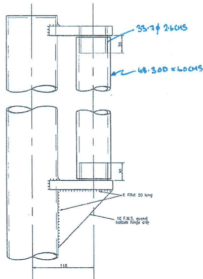
GATE CG1 - CG4 + CG6 HINGE DETAIL Scale 1:2
