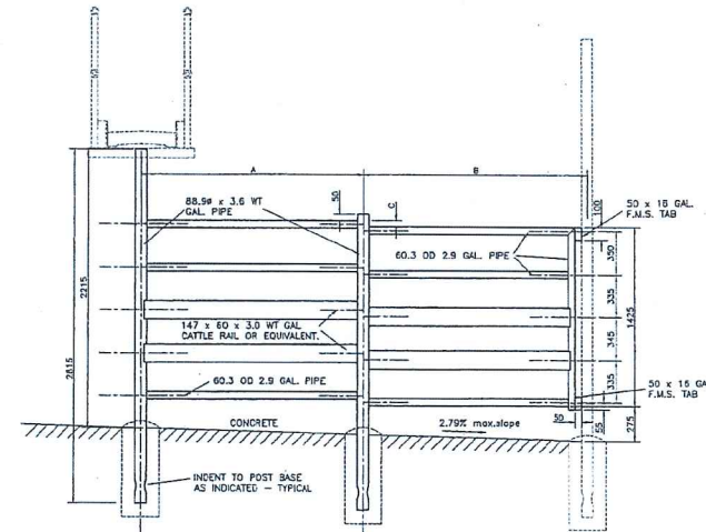
PANEL CP12A
