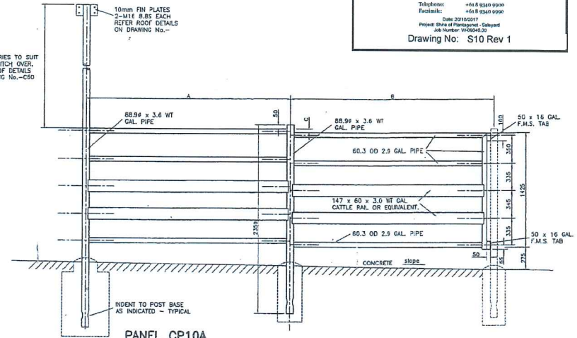
PANEL CP10A
