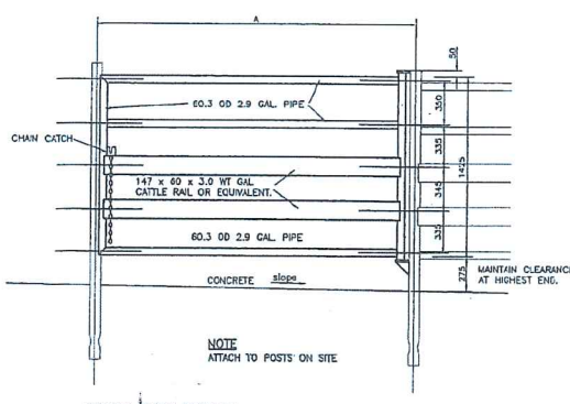
GATE CG1A - CG1C
