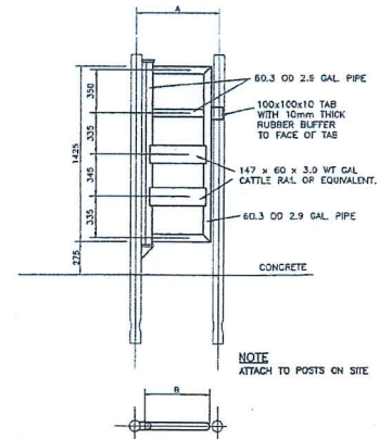
GATE CG5A - CG5G
