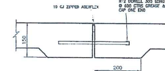
DOWEL JOINT DETAIL 'DJ'
