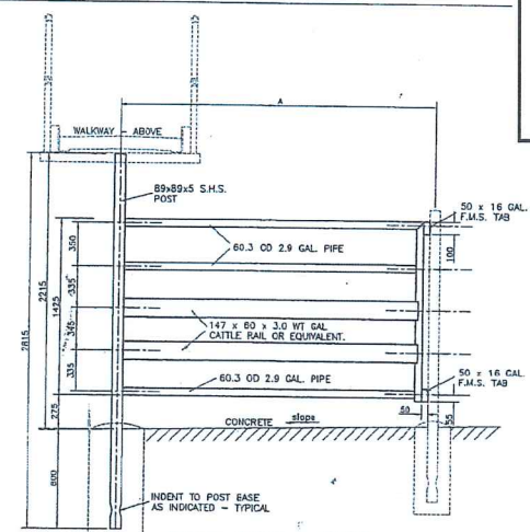
PANEL CP2A - CP2B
