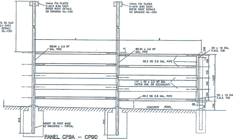
PANEL CP9A - CP9D
