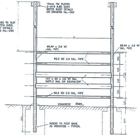
PANEL CP8A - CP8C
