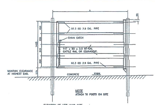
GATE CG3A - CG3C
