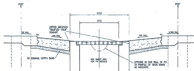
EFFLUENT COLLECTION POINT AT INVERT
