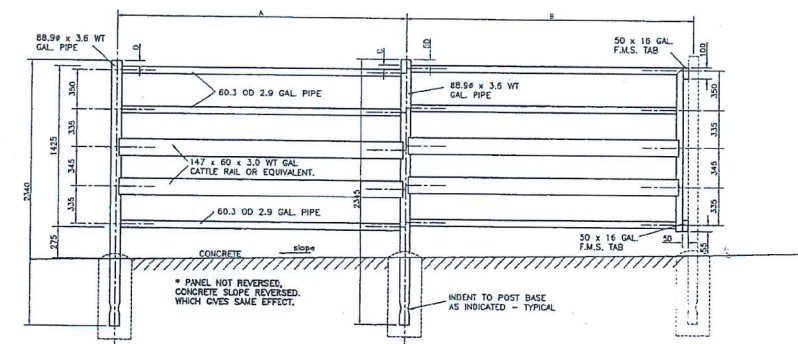
PANEL CP3A - CP3H REVERSED
